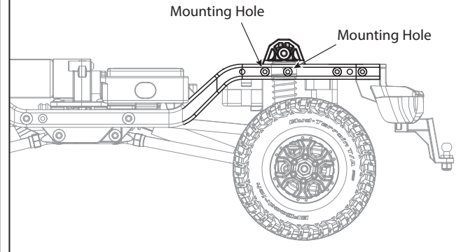
Rear Shock Tower Installation
